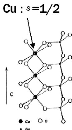
Fig.7 Crystal structure of CuGeO 3 .
