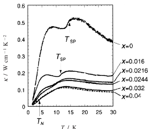
Fig.10 Thermal conductivity of \text{Cu}_{1-x}\text{Mg}_x\text{GeO}_3 in the direction of the spin chain with various Mg concentration x .
