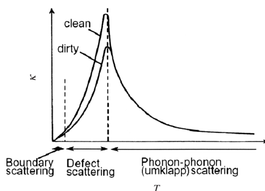
Fig.9 Typical temperature dependence of phonon thermal conductivity.
