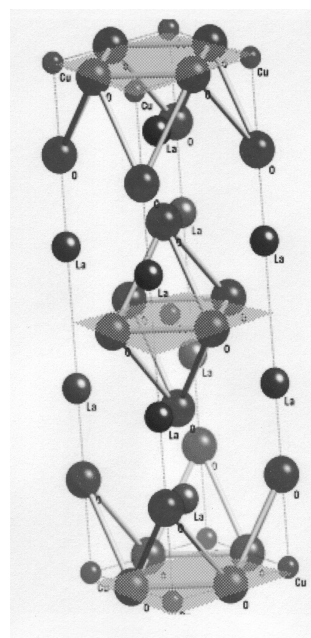
Fig.2 Crystal structure of La 2 CuO 4 .
