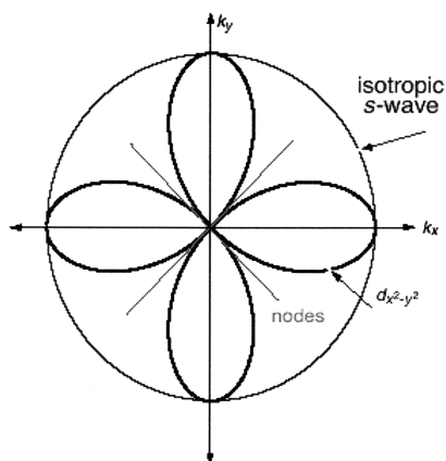
Fig.4 Schematic illustration of the s-wave and the d-wave pairing.
