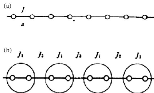
Fig.8 Schematic illustration of spin states for (a) disordered state and (b) the spin-Peierls state.
