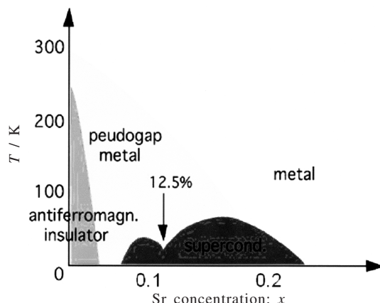
Fig.3 The phase diagram of a high- T_c cuprate superconductor \text{La}_{2-x}\text{Sr}_x\text{CuO}_4 .
