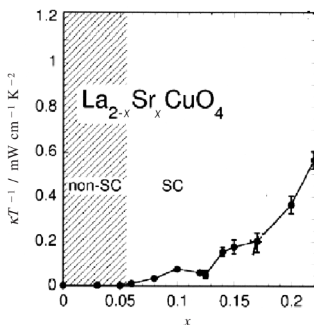
Fig.6 In-plane quasiparticle thermal conductivity of \text{La}_{2-x}\text{Sr}_x\text{CuO}_4 as function of x .
