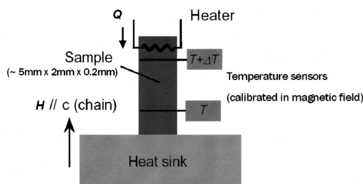
Fig.1 Schematic illustration of the thermal conductivity measurement.
